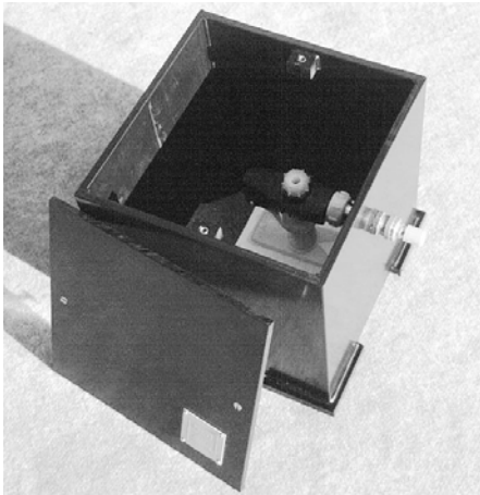
Inspection chamber/Irrigation unit for intensive green roof build-ups.
